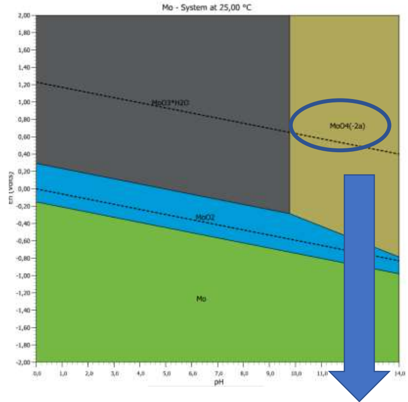
Figure 2: E-pH diagram for system Mo-H 2 O at 25°C.
