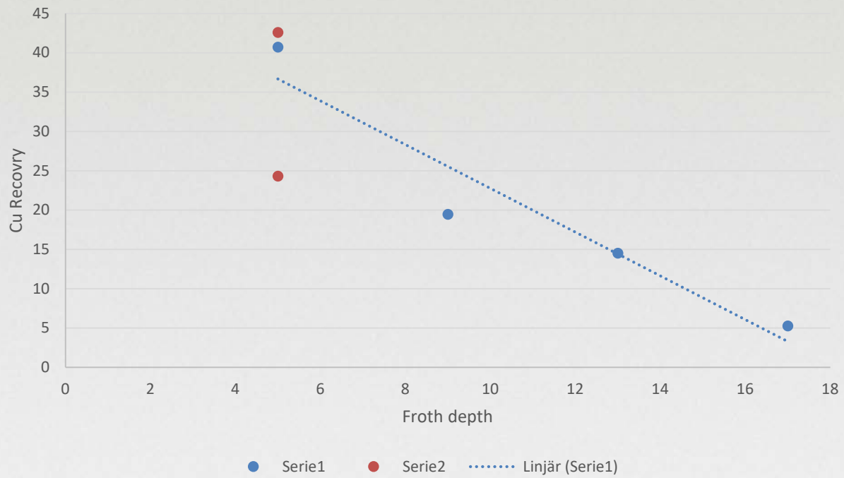
Cu recovery in concentrate
